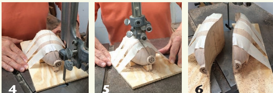
The author's pod cut in half on a curved line. The tenons at each end can be cut off after the pod is split.
